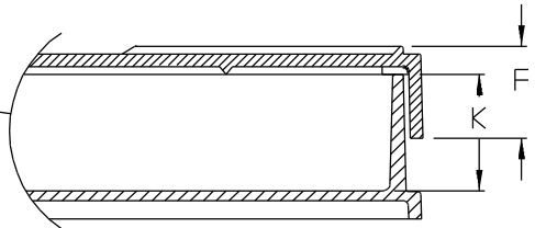
CORNER DETAIL
