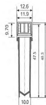
81-8204&81-7205 Dimensions=mm
