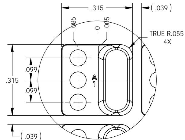
DETAIL G SCALE 6 : 1 96X
