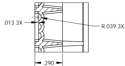
DETAIL E SCALE 3 : 1
